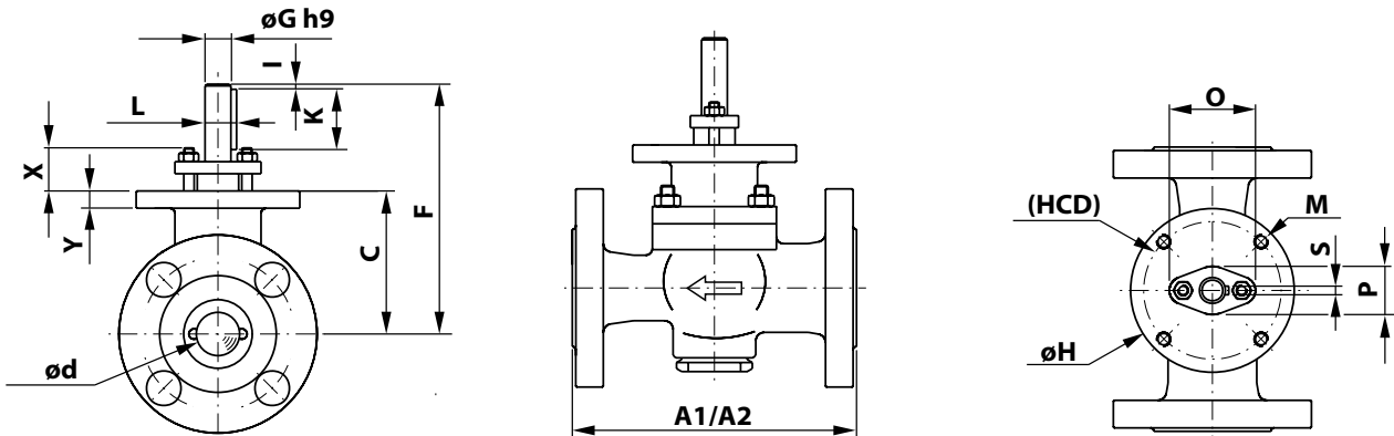
Ball segment valve type KVTF/KVXF
